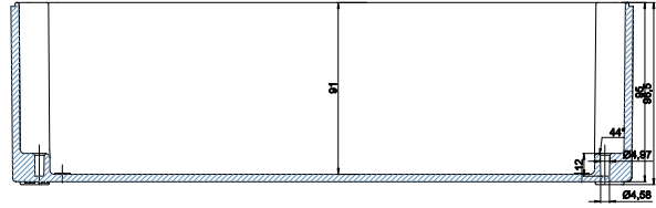
SECTION C-C
